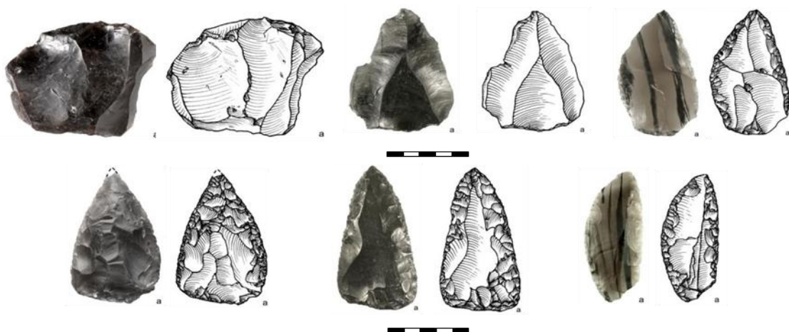
Selected artifacts from Barozh-12: 1 Levallois core; 2 Levallois point; 3 Double straight-convex scraper; 4 Mousterian point; 5 Convergent scraper; 6 Double straight-convex scraper (modified after Glauberman et al. 2020a)
